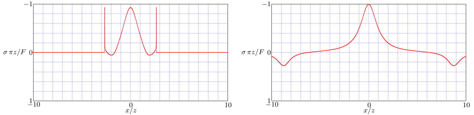
Figure 11.18: Line Load - Isotropic Stress, \nu = 0 , c_s t / z = 2 and \nu = 0 , c_s t / z = 10 .
