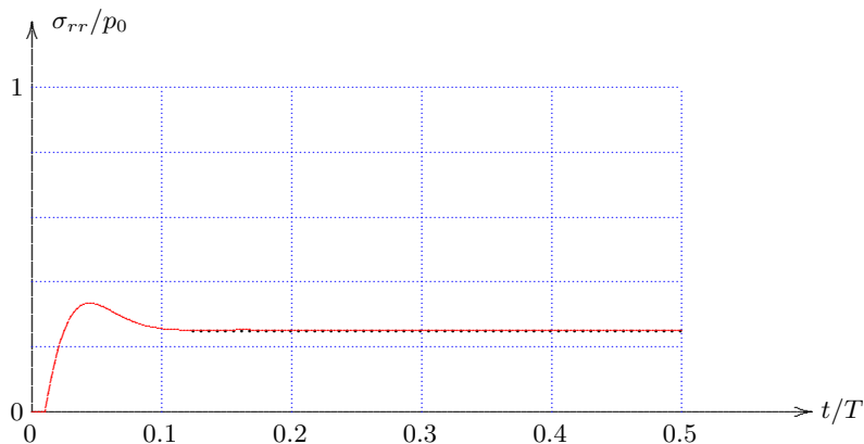
Figure 6.14: Radial stress, cT/a = 100 , \nu = 0.25 , r/a = 2 .
