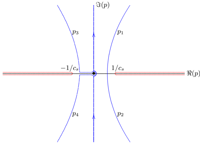
Figure 10.4: Transformed integration paths, for x < 0 and x > 0 .
