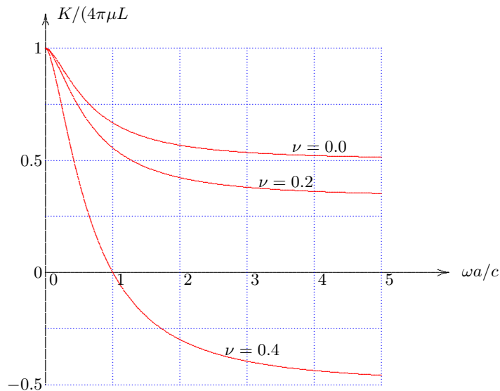
Figure 6.10: Equivalent spring.
