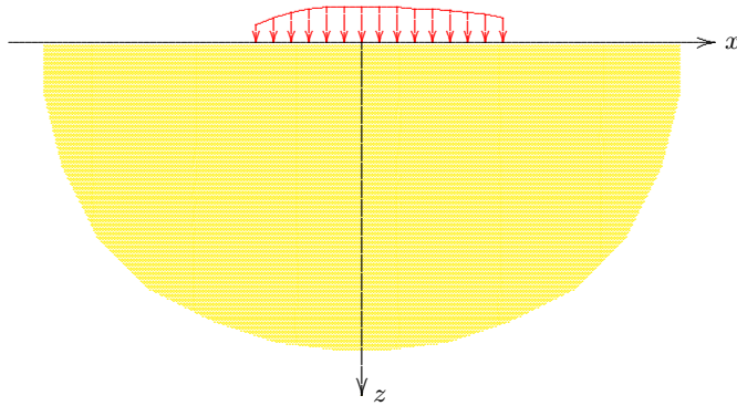
Figure 8.3: Boussinesq problem.
