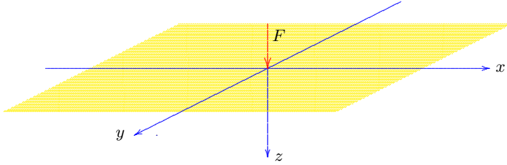
Figure 10.8: Point load on half space.
