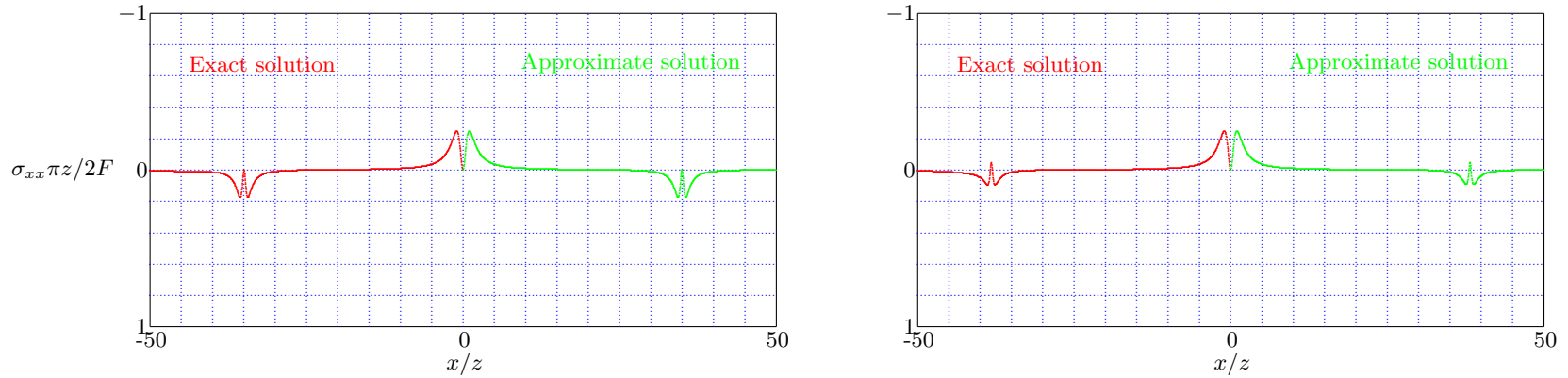
Figure 11.27: Line Load - Horizontal Normal Stress, c_s t/z = 40 , \nu = 0 and \nu = 0.5 .
