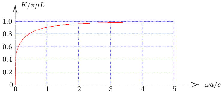
Figure 6.16: Equivalent spring.
