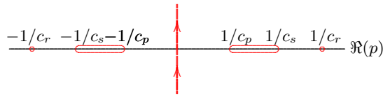
Figure 11.10: Branch cuts in the p -plane.
