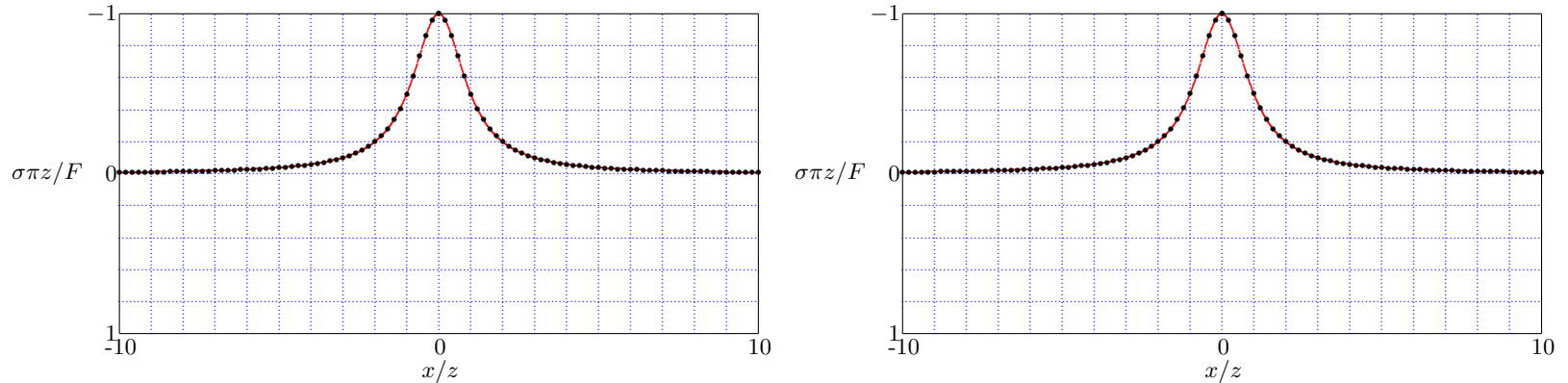
Figure 11.19: Line Load - Isotropic Stress, \nu = 0 , c_s t / z = 20 and \nu = 0.5 , c_s t / z = 20 .
