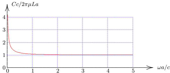
Figure 6.17: Equivalent damping.
