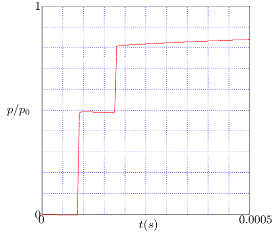
Figure 5.3: Shock wave in a porous medium - Analytical solution.
