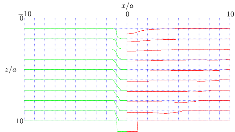
Figure 10.7: Stresses below a strip load, \nu = 0.499 , c_p t/a = 10 .
