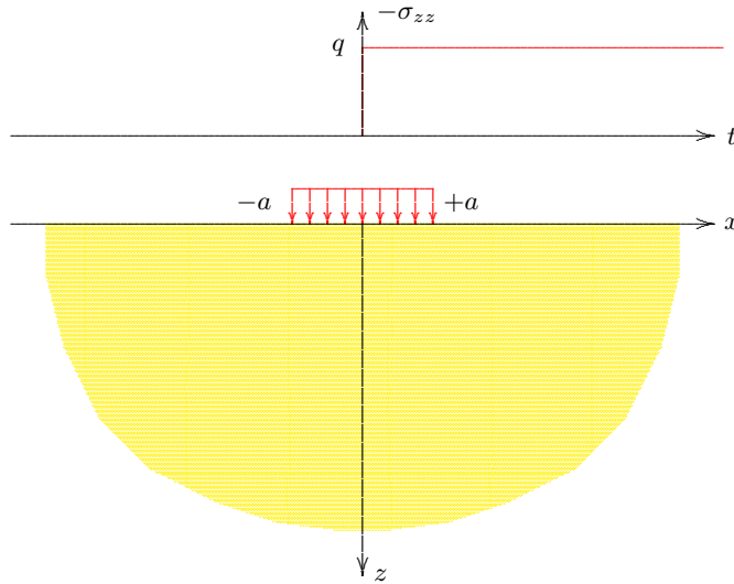
Figure 10.5: Half plane with strip load.
