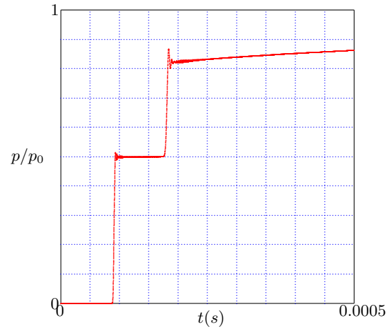
Figure 5.4: Shock wave in a porous medium - Numerical solution.
