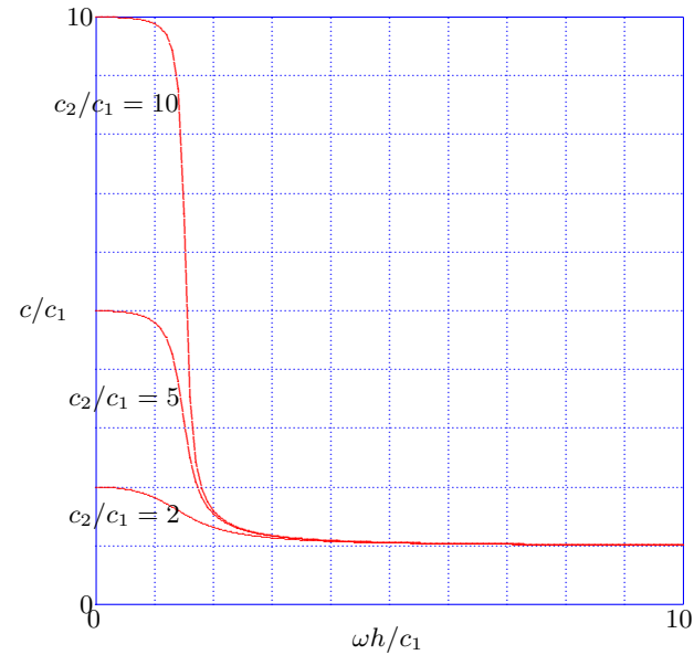
Figure 9.6: Velocity of Love wave.
