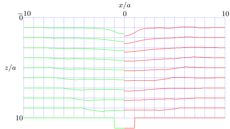
Figure 10.6: Stresses below a strip load, \nu = 0 , c_p t/a = 10 .
