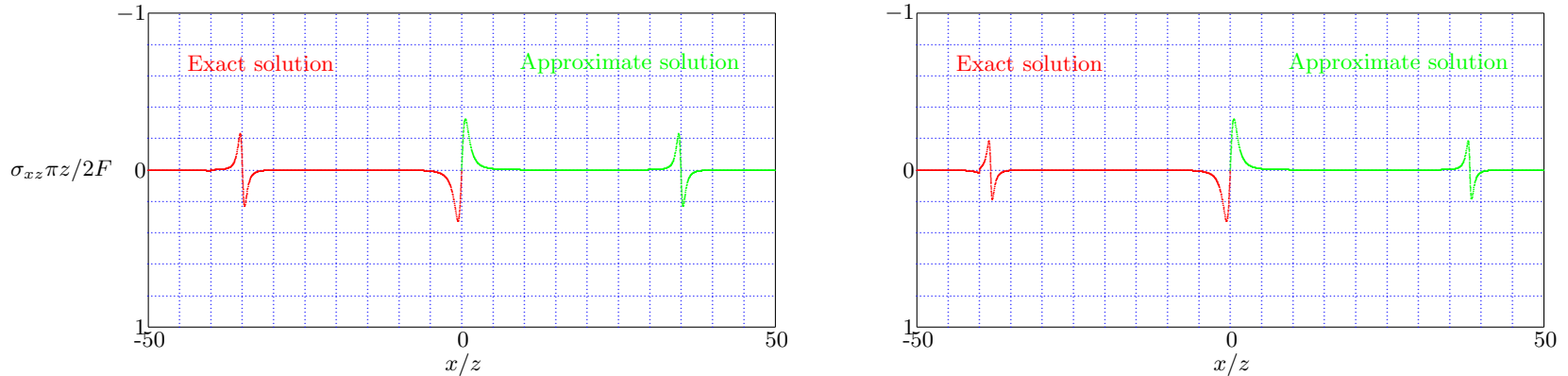
Figure 11.30: Line Load - Shear Stress, c_s t/z = 40 , \nu = 0 and \nu = 0.5 .
