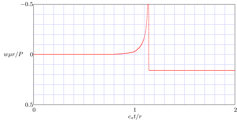
Figure 13.4: Vertical displacement, \nu = 0.00 .
