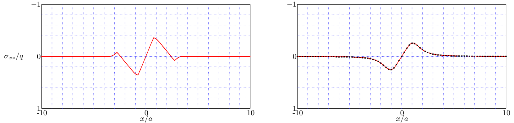
Figure 12.18: Strip Load - Shear Stress, \nu = 0.0 , z/a = 1 ; c_st/a = 2 (left) and c_st/a = 20 (right).
